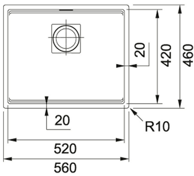
Technical Drawing
